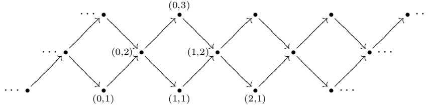
FIGURE 3. The quiver \vec{\mathbb{Z}}\vec{\Delta} for \vec{\Delta} of type A_3 . The vertices in \text{mod } A are labeled.
